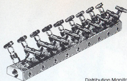
Distribution Manifold 20 Outlets max.
